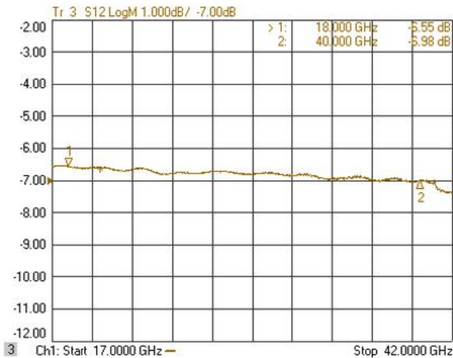
3. 插入损耗 Insertion Loss
